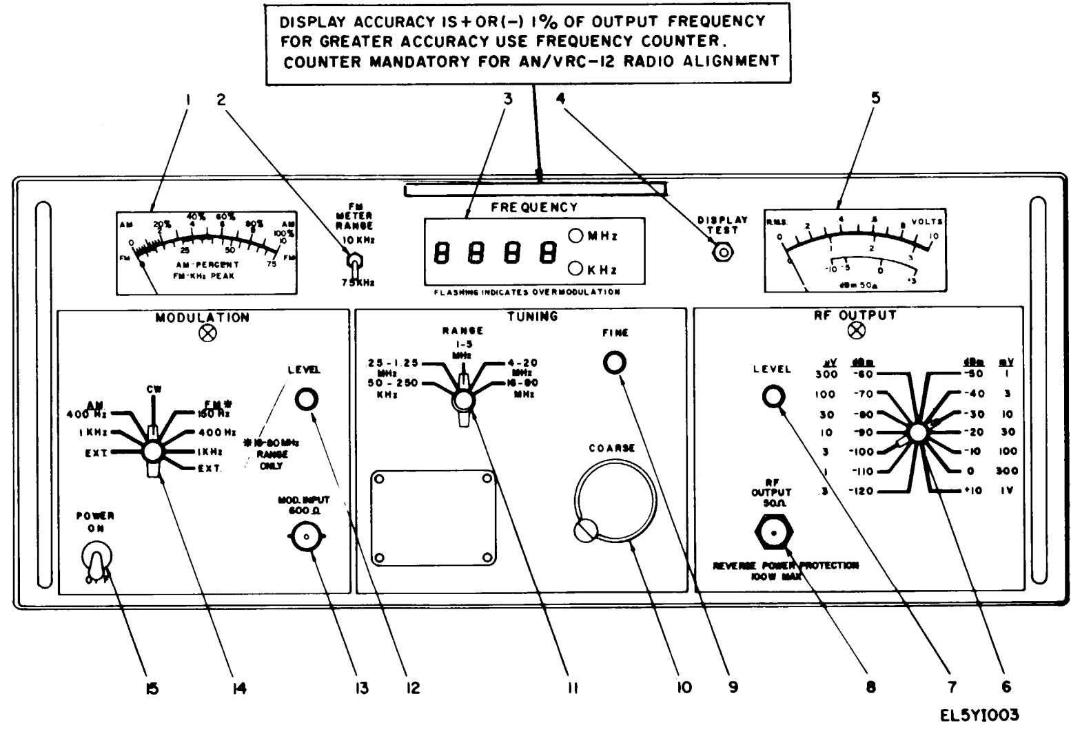
Figure 3-1. Operator's Controls and Indicators.
