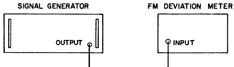
FIG 9-9. TEST SETUP, DEVIATION ACCUARACY
