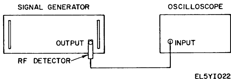
FIG 9-12. TEST SETUP, SPURIOUS AM
