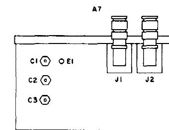
VIEW H-H
